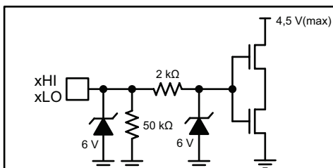
Figure 4c: xHI, xLO Inputs
