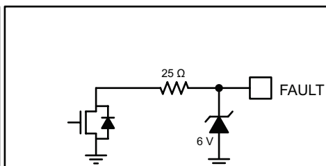
Figure 4e: FAULT Output
