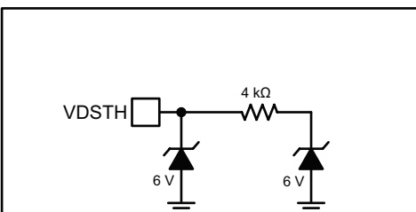
Figure 4d: VDSTH Input
