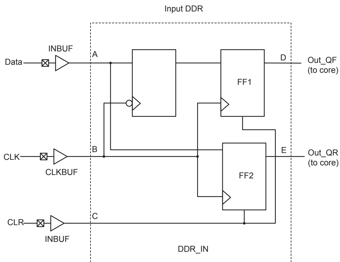
Figure 2-15 • Input DDR Timing Model
