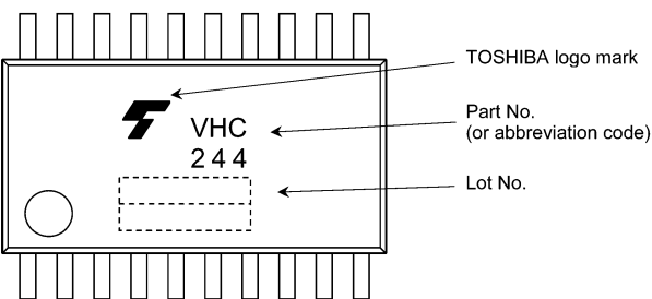
74VHC244FT
