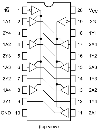
74VHC244FT
