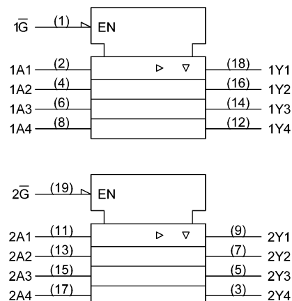
74VHC244FT
