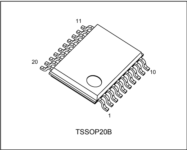
74VHC244FT
