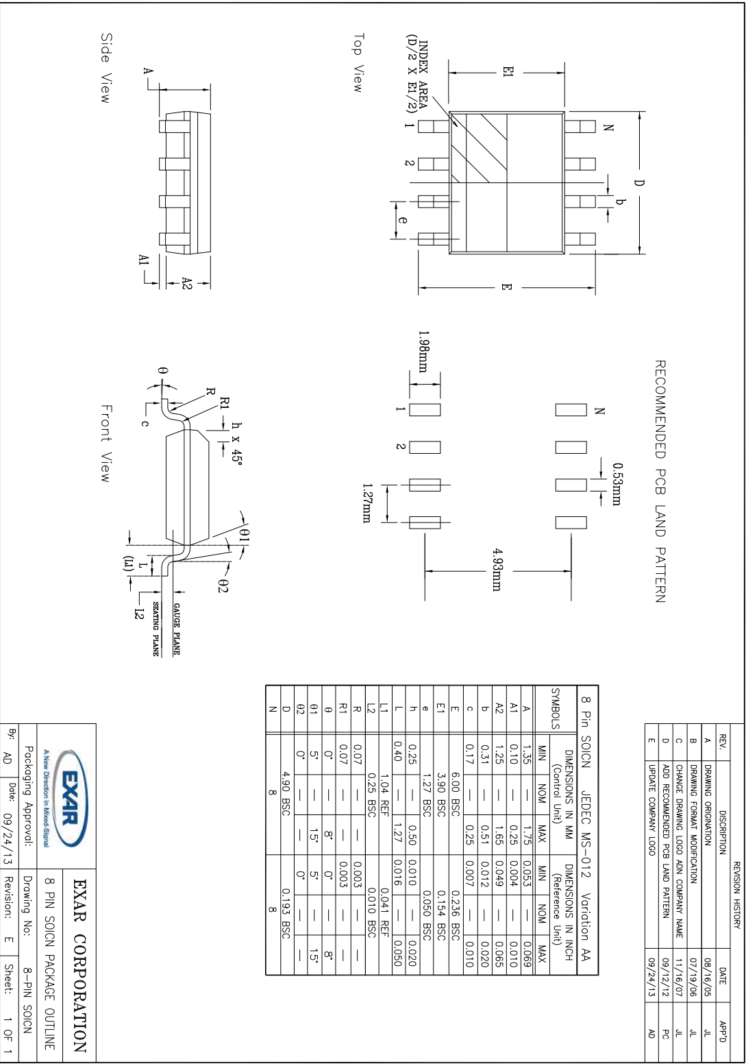
FIGURE 11. 8 NSOIC
