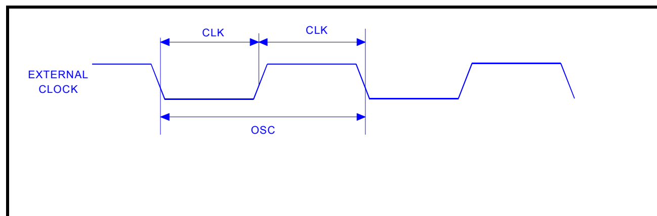
FIGURE 14. CLOCK TIMING
