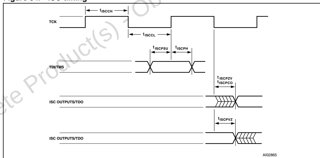
Figure 84. ISC timing
