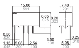
External dimensions Standard PC board terminal
