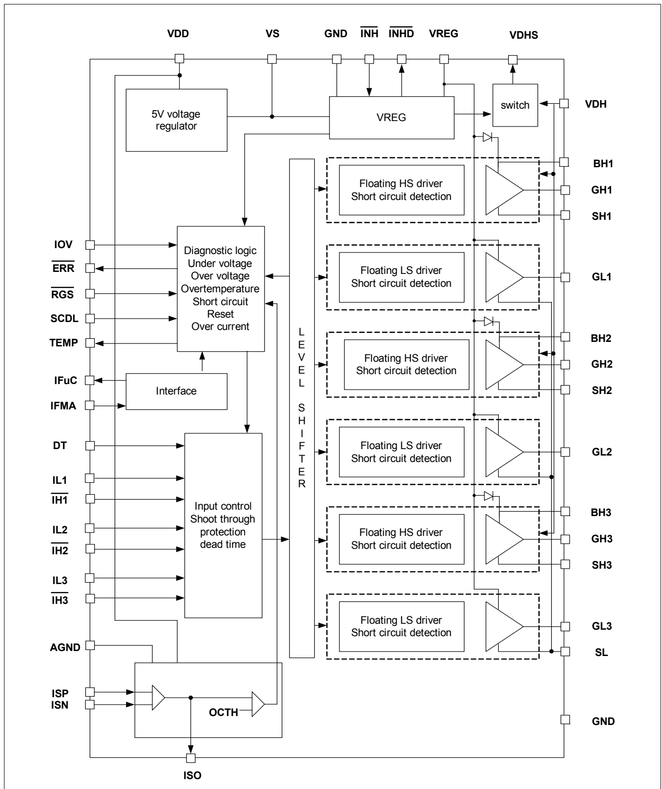
Figure 1 Block Diagram
