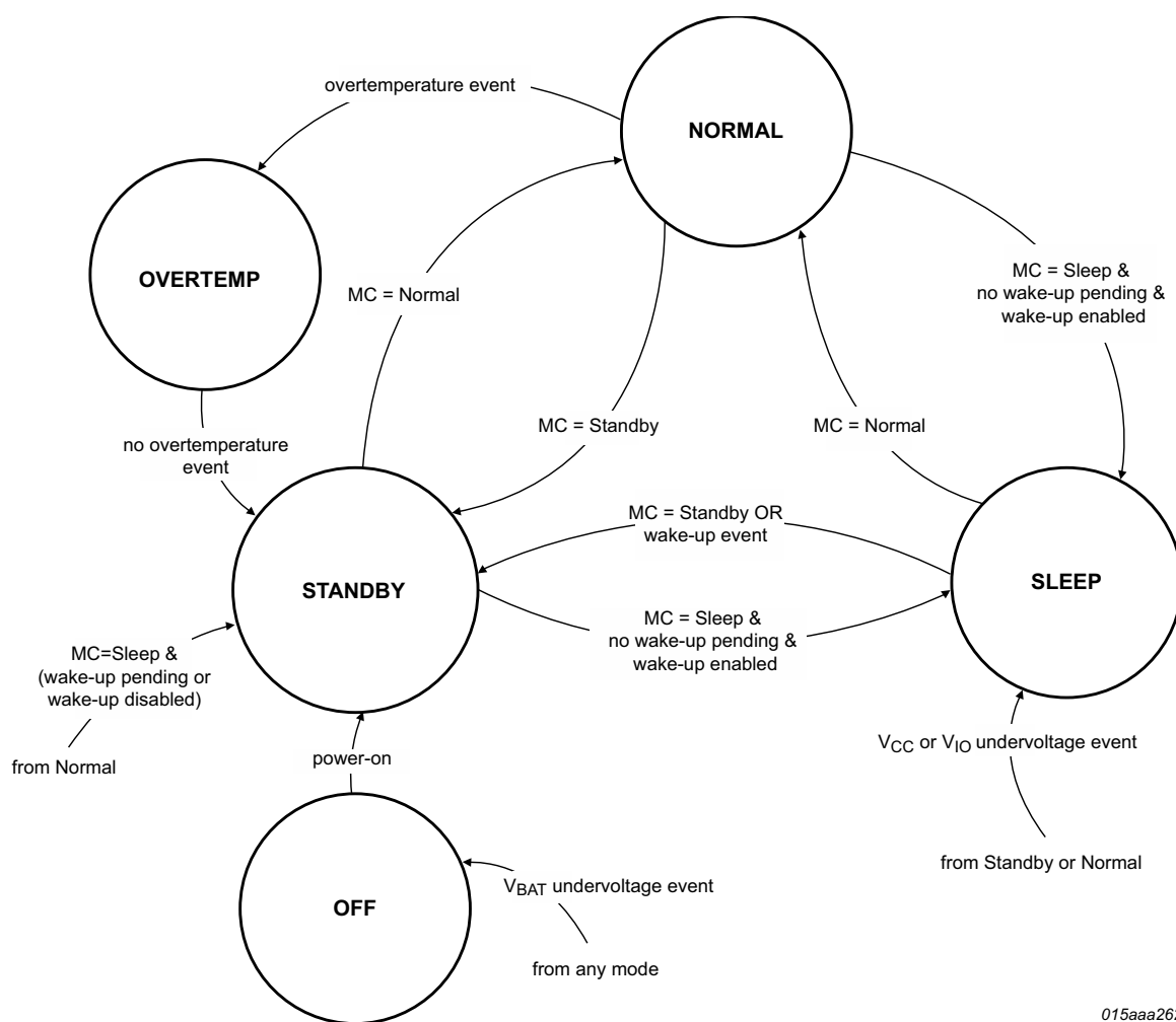
Fig 4. TJA1145 system controller state diagram
