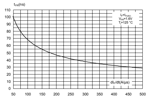
Figure 10. Forward recovery time versus di_F/dt (typical values)
