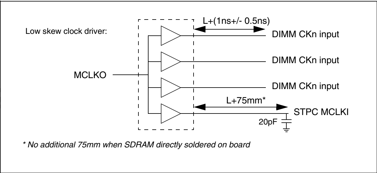
Figure 6-23. Clock Routing
