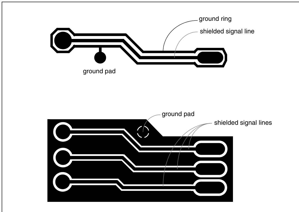
Figure 6-20. Shielding signals
