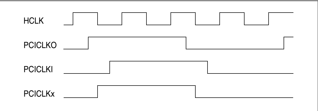
Figure 6-30. Clocks relationships
