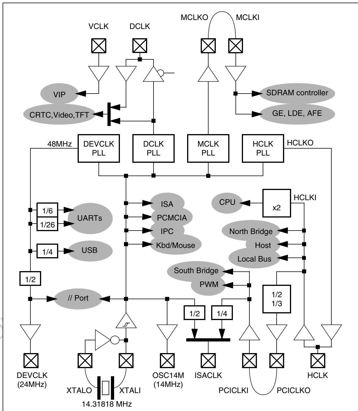
Figure 1-2. STPC Atlas clock architecture
