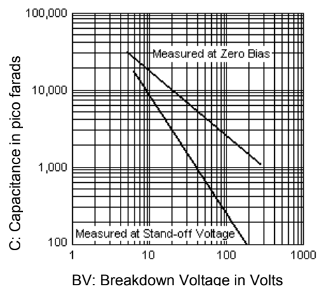
FIGURE 4 Typical Capacitance vs. Breakdown Voltage
