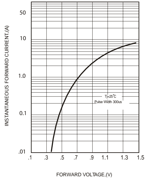
FIG.7-TYPICAL FORWARD CHARACTERISTICS
