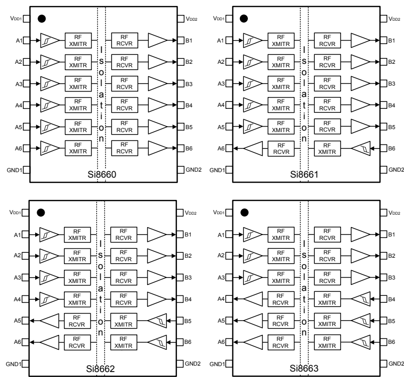
Figure 5.1. Si866x Pinout
