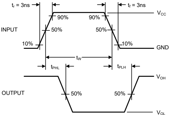
Figure 2. AC Waveforms
