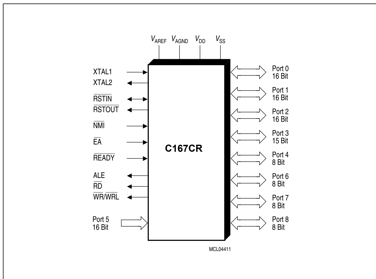
Figure 1 Logic Symbol
