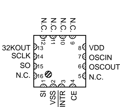
R2043L(QFN023023-16)
