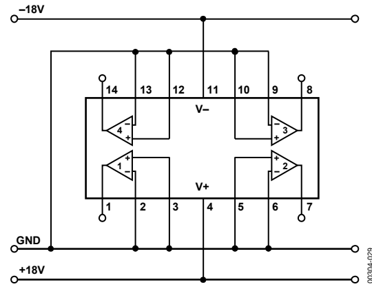
Figure 30. Burn-In Circuit
