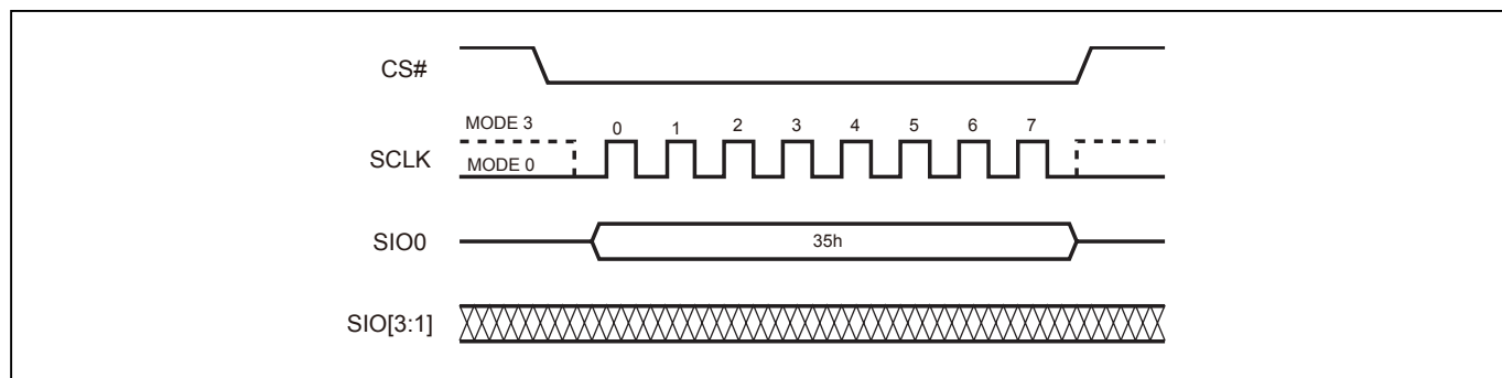
Figure 7. Enable QPI Sequence
