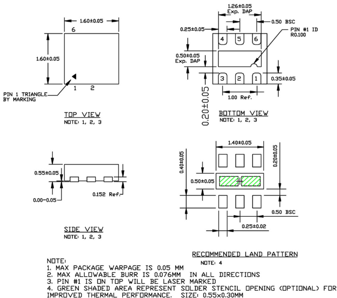
6-Pin 1.6mm × 1.6mm TDFN (MT)
