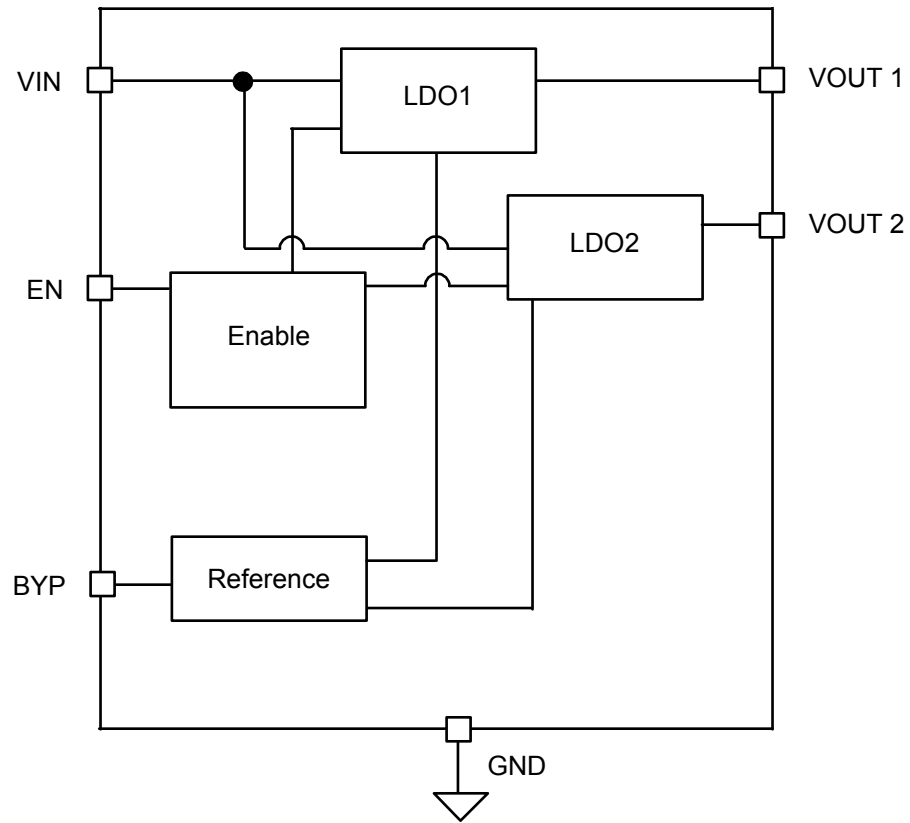
MIC5321 Block Diagram
