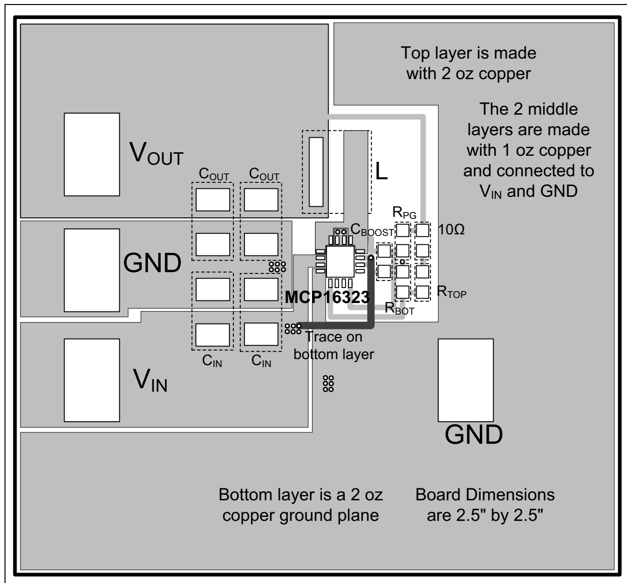
FIGURE 5-1: Recommended Layout.
