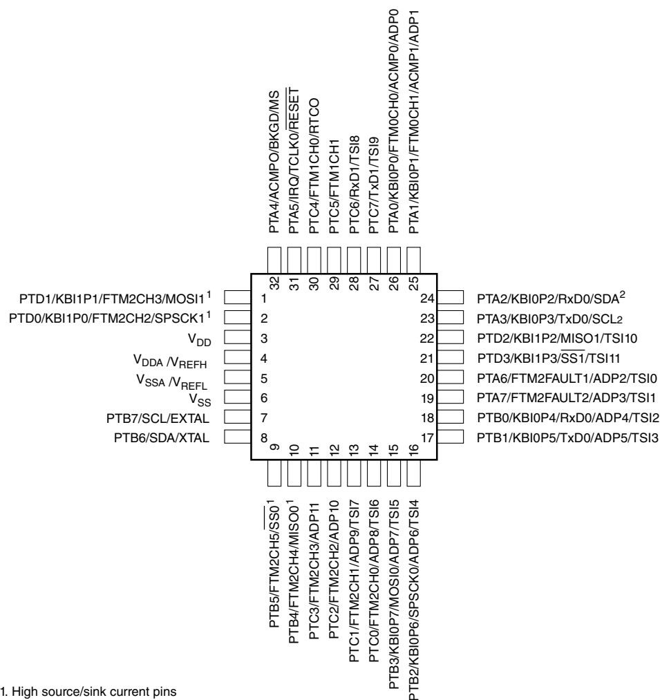
Figure 25. MC9S08PT60 32-pin LQFP package
