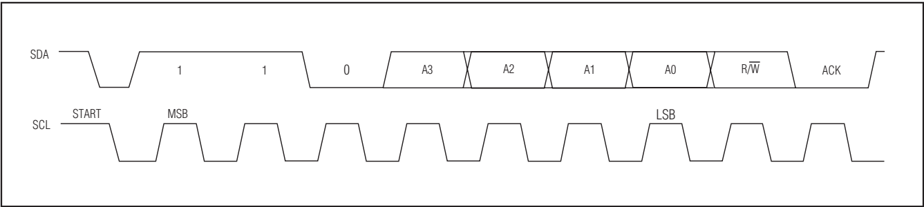
Figure 4. Slave Address
