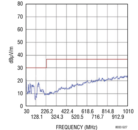
Radiated Emissions, 36V_{IN} , 24V_{OUT} at 1.5A Load
