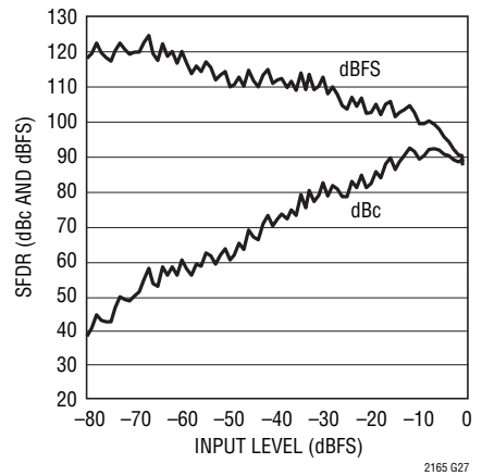
LTC2163 SFDR vs Input Level, f_{IN} = 70\text{MHz} , 2\text{V} Range, 80Msps
