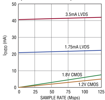
LTC2165 I_{OVPD} vs Sample Rate, 5MHz Sine Wave Input, -1dBFS, 5pF on Each Data Output
