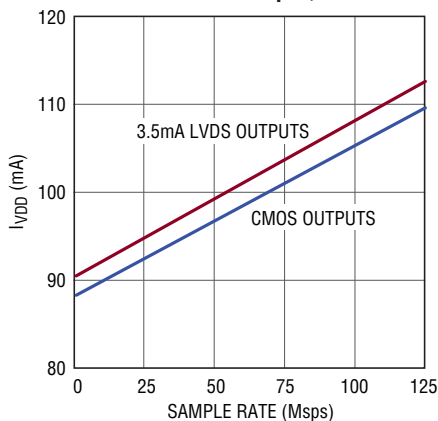
LTC2165 I_{VDD} vs Sample Rate, 5MHz Sine Wave Input, -1dBFS
