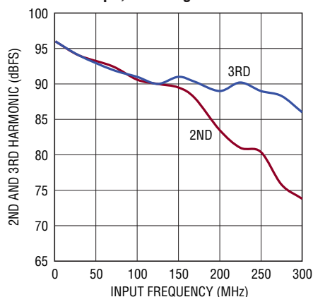
LTC2165: 2nd, 3rd Harmonic vs Input Frequency, -1dBFS, 125Msps, 1V Range
