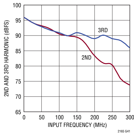
LTC2163 2nd, 3rd Harmonic vs Input Frequency, -1\text{dBFS} , 80Msps, 1\text{V} Range
