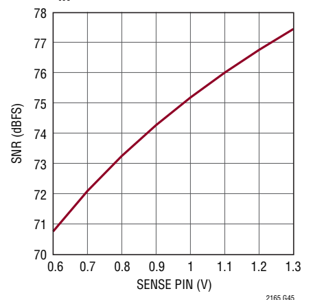
LTC2163 SNR vs SENSE, f_{IN} = 5\text{MHz} , -1\text{dBFS}
