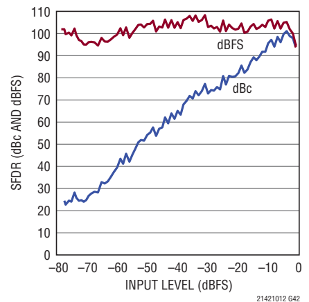
LTC2140-12: SFDR vs Input Level, f_{IN} = 70\text{MHz} , 25Mps, 2V Range
