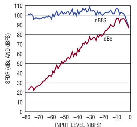
LTC2141-12: SFDR vs Input Level, f_{IN} = 70\text{MHz} , 40Msps, 2V Range
