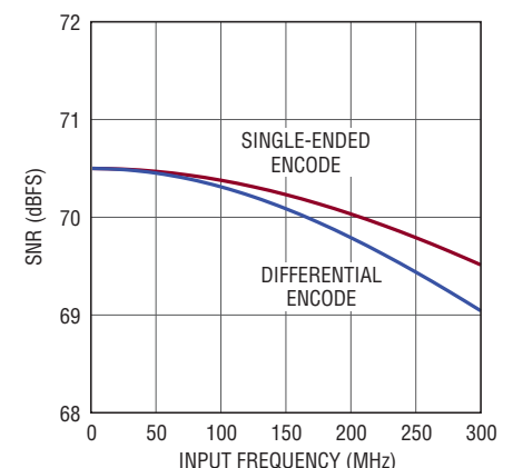
LTC2141-12: SNR vs Input Frequency, -1\text{dBFS} , 40Msps, 2V Range
