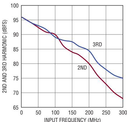
LTC2141-12: 2nd, 3rd Harmonic vs Input Frequency, -1\text{dBFS} , 40Msps, 2V Range
