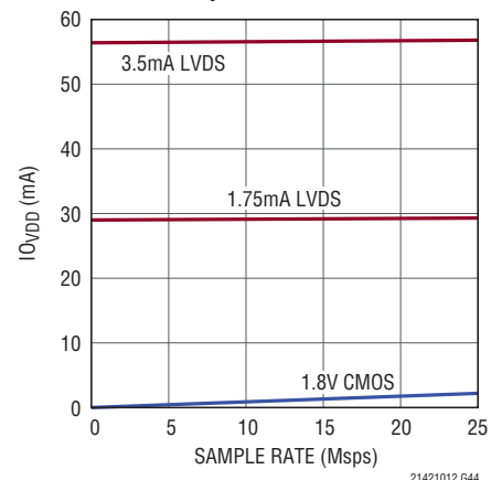
LTC2140-12: I_{O_VDD} vs Sample Rate, 5MHz, -1dBFS, Sine Wave on Each Input
