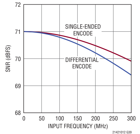
LTC2140-12: SNR vs Input Frequency, -1dBFS, 25Mps, 2V Range
