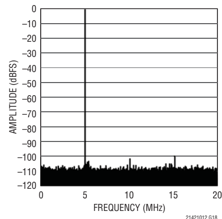
LTC2141-12: 64k Point FFT, f_{IN} = 5\text{MHz} , -1dBFS, 40Msps
