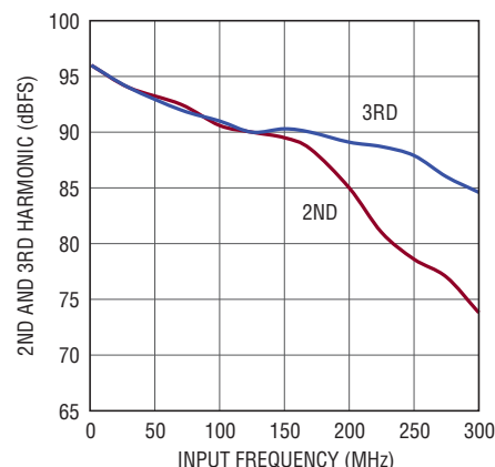
LTC2141-12: 2nd, 3rd Harmonic vs Input Frequency, -1\text{dBFS} , 40Msps, 1V Range
