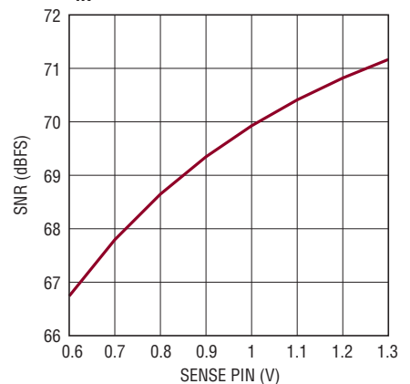
LTC2140-12: SNR vs SENSE, f_{IN} = 5\text{MHz} , -1dBFS
