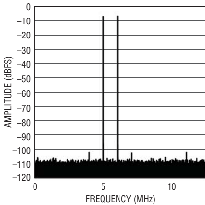
LTC2140-12: 64k Point 2-Tone FFT, f_{IN} = 69\text{MHz} , 70\text{MHz} , -7dBFS, 25Mps
