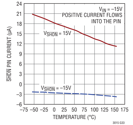
\overline{\text{SHDN}} Pin Input Current
