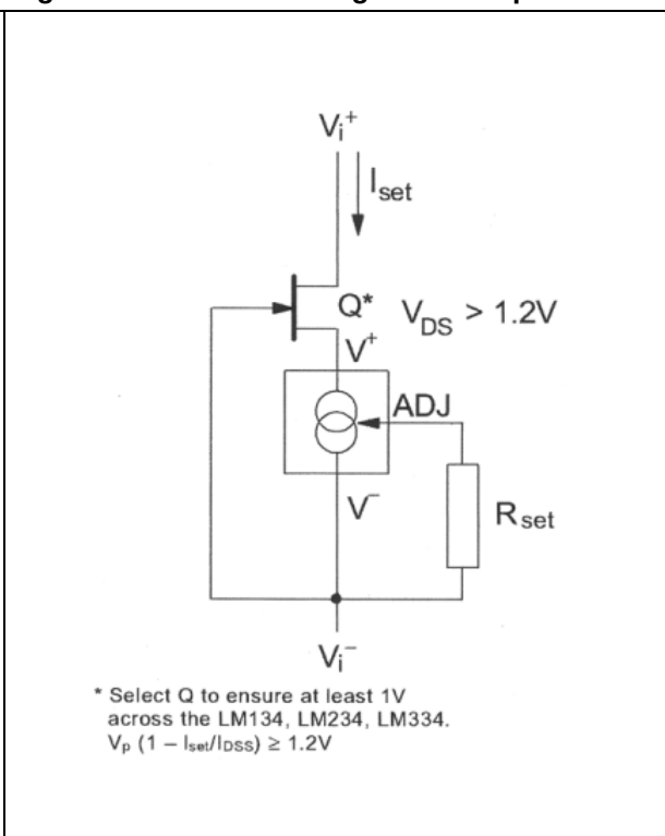
Figure 20. Fet cascading for low capacitance
