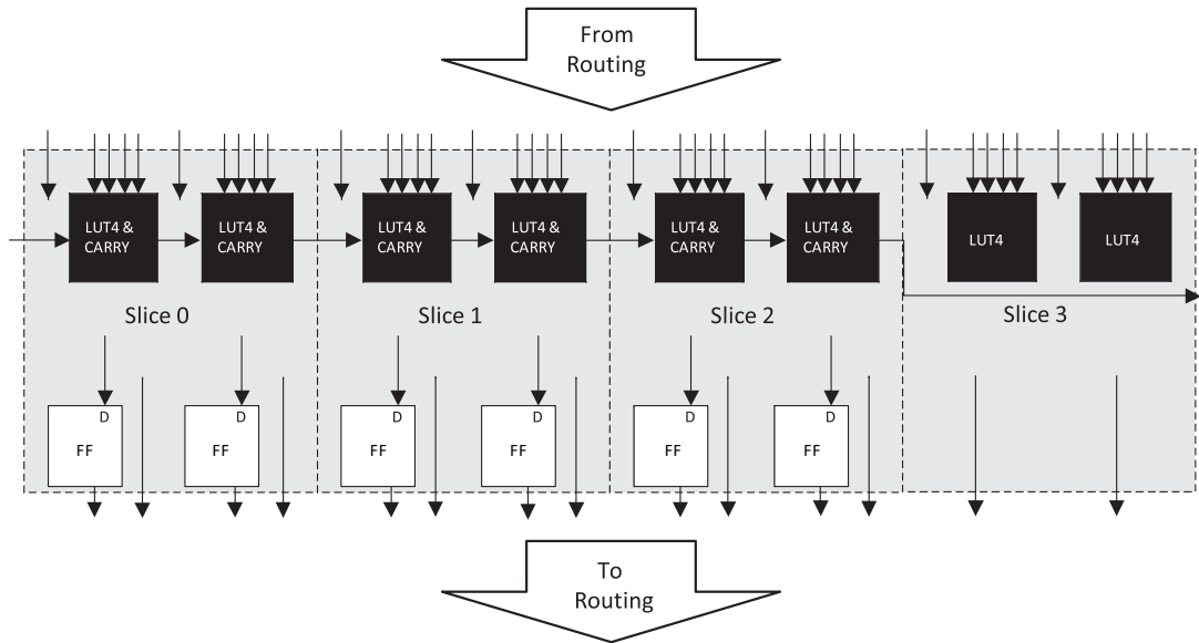
Figure 2.2. PFU Diagram
