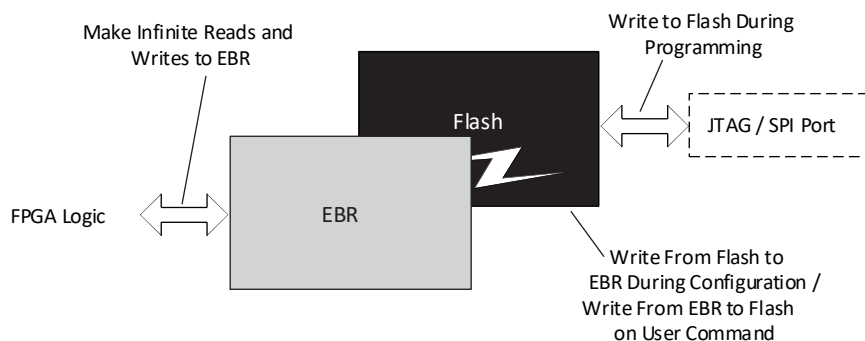
Figure 2.16. FlashBAK Technology
