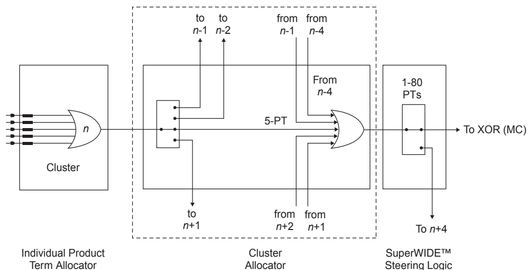
Figure 4. Macrocell Slice
