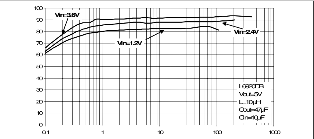
Figure 3. Efficiency vs output current @ V_{OUT} = 5V
