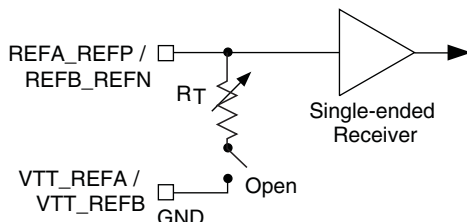
Figure 3-15. LVCMOS/LVTTTL Input Receiver Configuration
