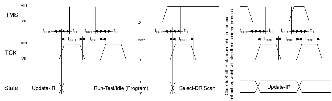
Figure 3-10. Verify Timing Diagram
