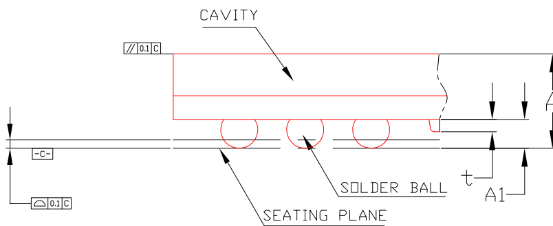
DETAIL : "A"
