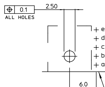
PCB-HOLE LAYOUT COMPONENT SIDE
