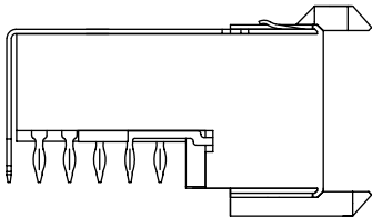
HM2R65PA5108N9 (top shielded only, 4 mm pitch)
