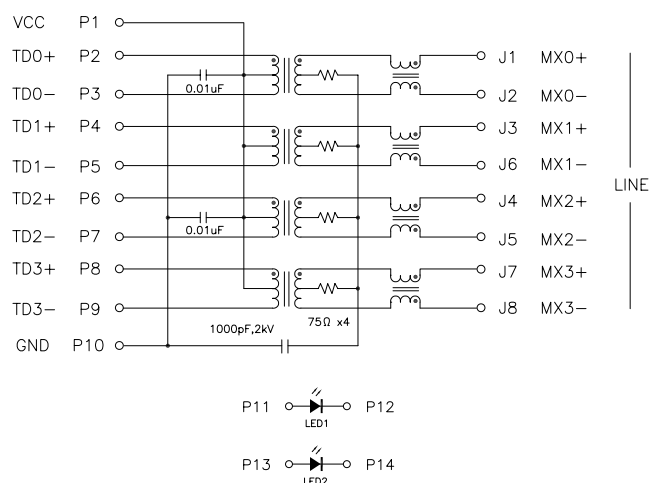
Circuit E
