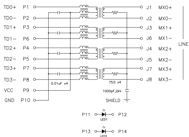
Circuit D
