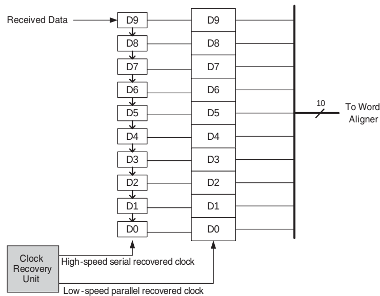
Figure 2-14. Deserializer (Note 1)
