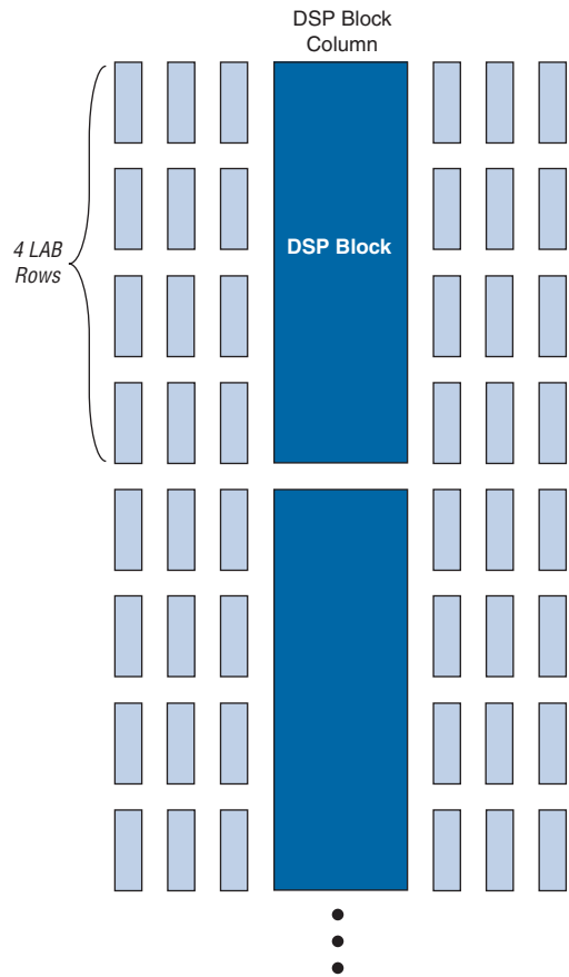
Figure 2-50. DSP Blocks Arranged in Columns
