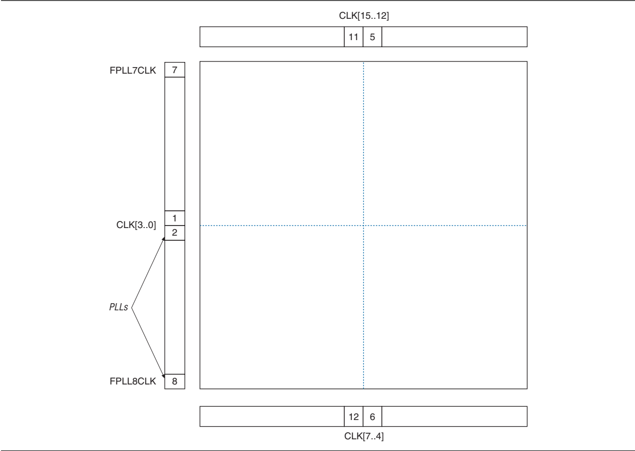
Figure 2-61. PLL Locations
