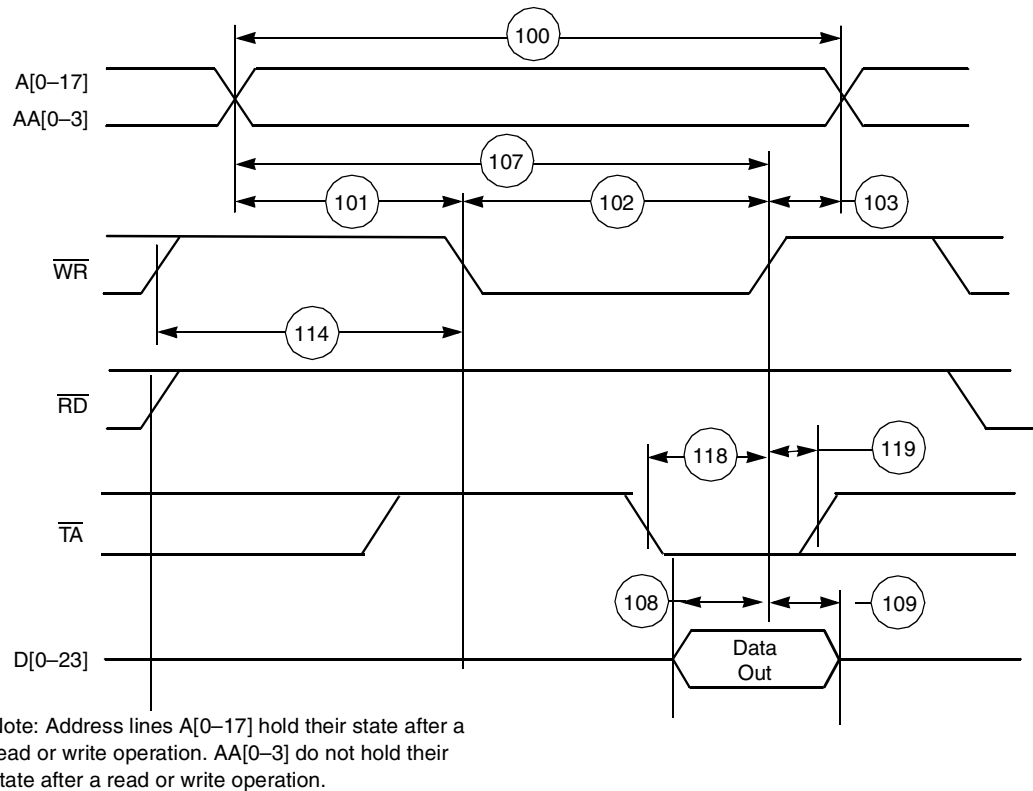
Figure 2-11. SRAM Write Access
