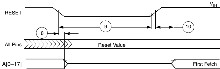
Figure 2-3. Reset Timing
