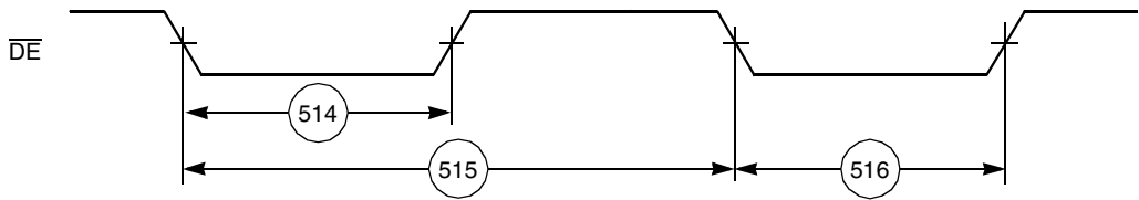
Figure 2-39. OnCE—Debug Request
