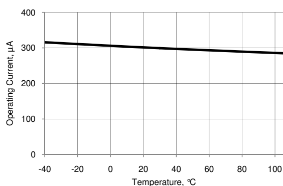
Figure 11-63. VDAC Operating Current vs Temperature, 1 V Mode, Fast Mode
