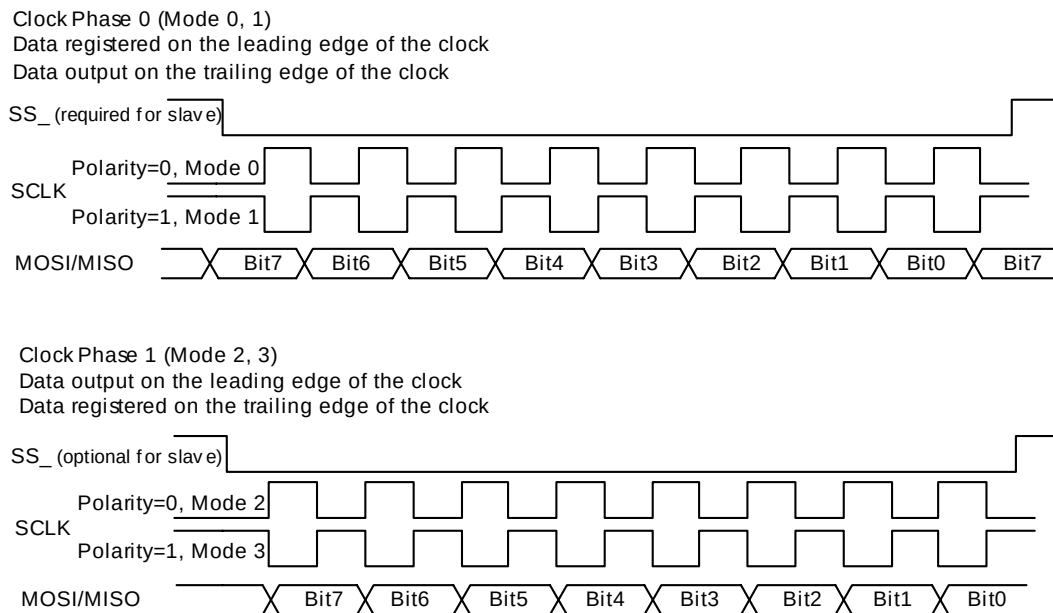
Figure 15: SPI Waveforms
