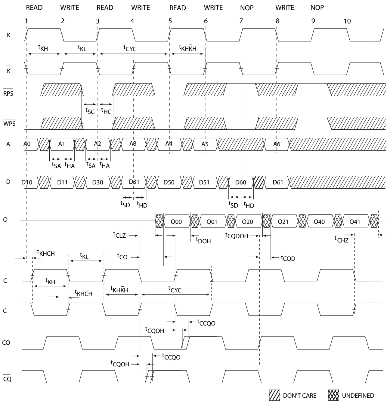
Figure 5. Read/Write/Deselect Sequence [26, 27, 28]
