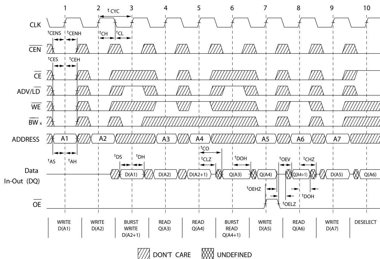
Figure 5. Read/Write Timing [27, 28, 29]
