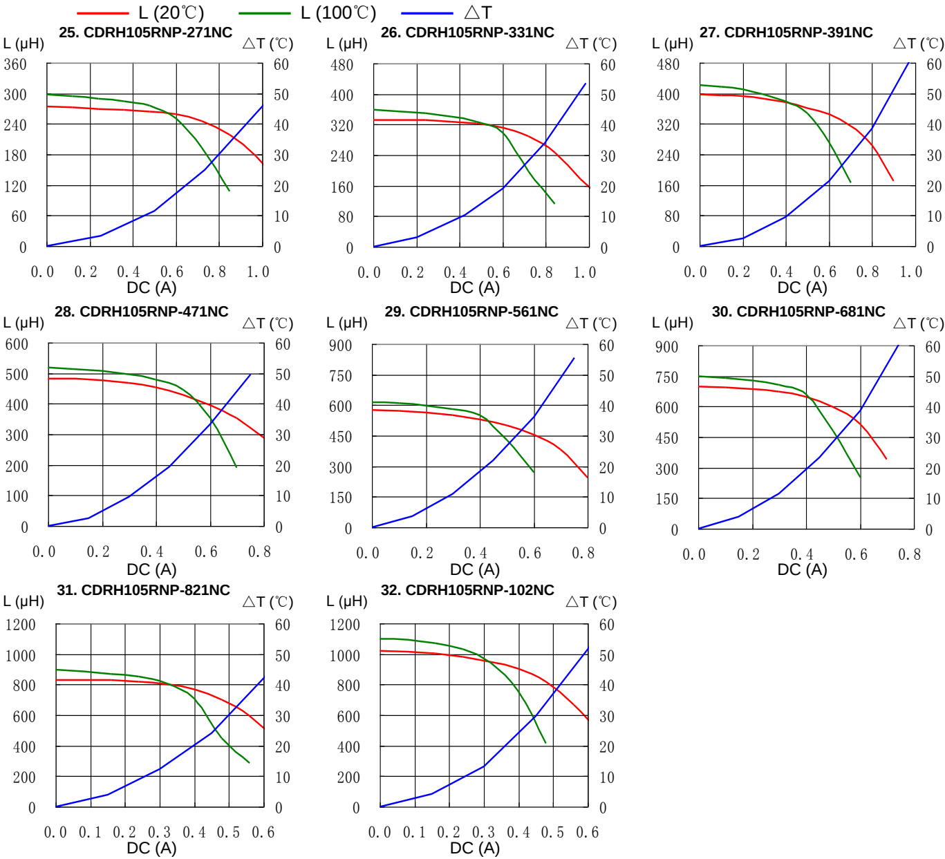
Saturation Current & Temperature Rise Graph
