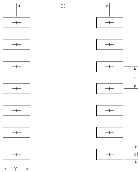
Figure 4.7. SOIC-14 PCB Land Pattern
