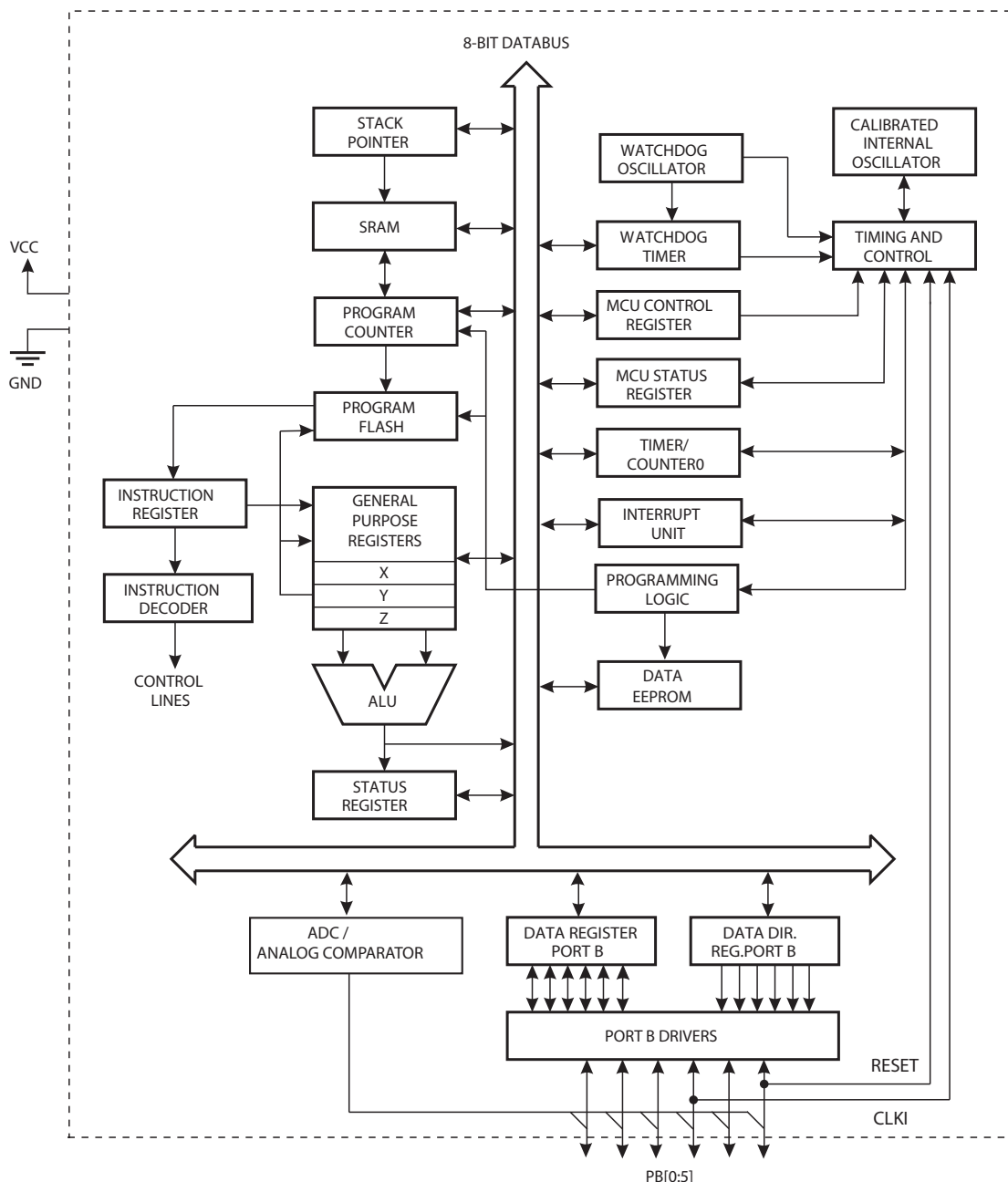
Figure 2-1. Block Diagram
