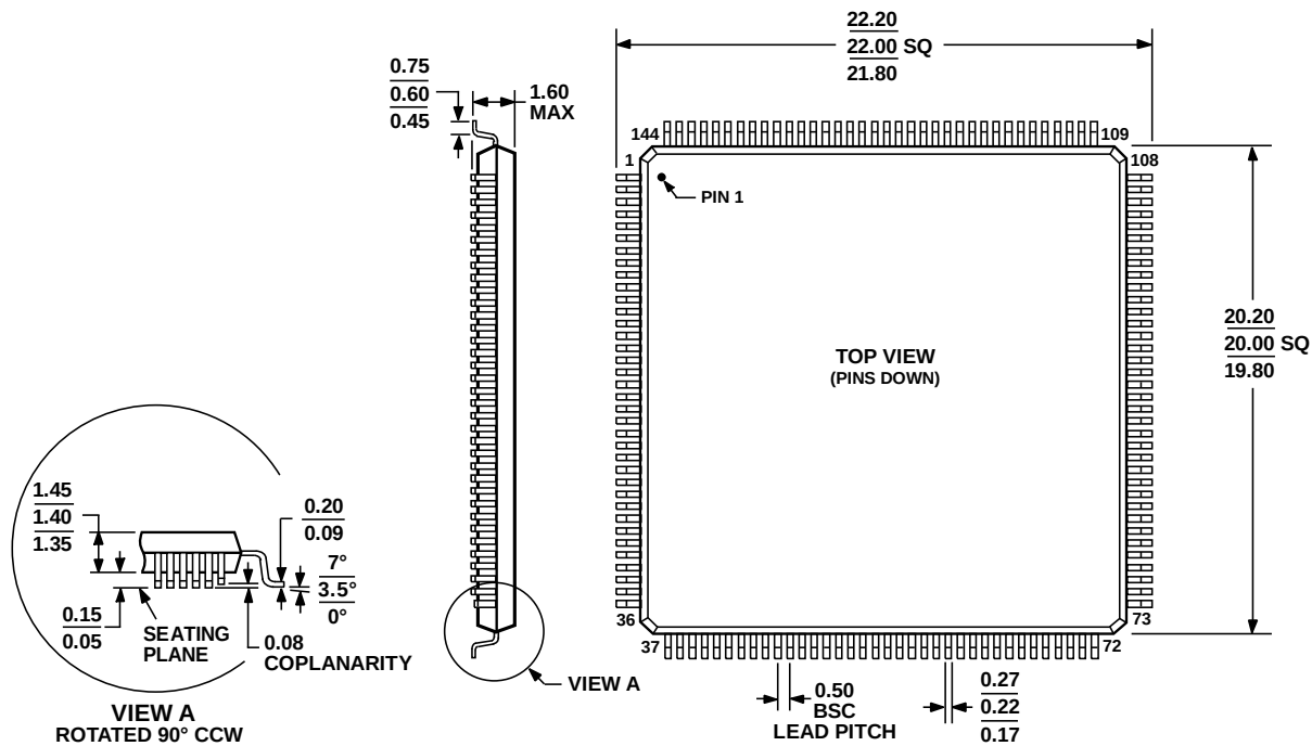
COMPLIANT TO JEDEC STANDARDS MS-026-BFB Figure 6. 144-Lead Low Profile Quad Flat Package [LQFP] (ST-144) Dimensions shown in millimeters
