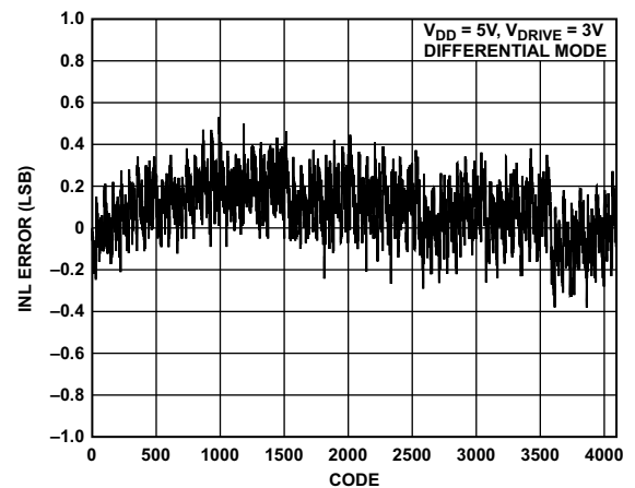
Figure 55. Typical INL
