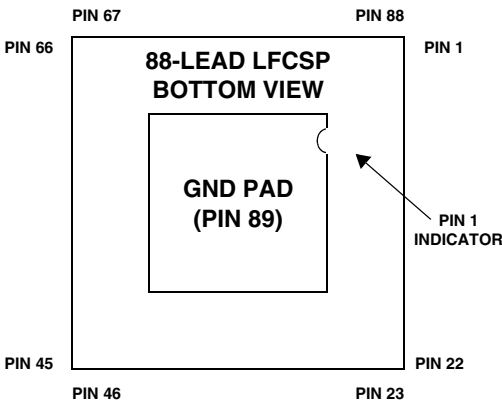
Figure 92. 88-Lead LFCSP Lead Configuration (Bottom View)
