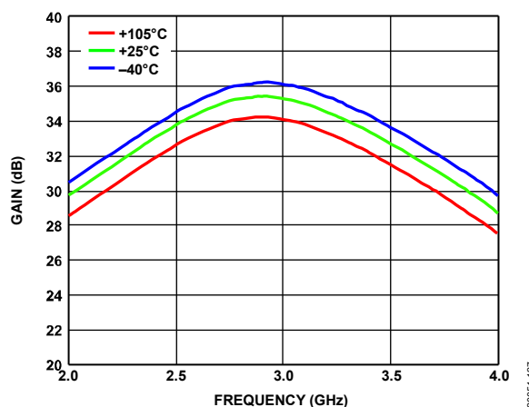
Figure 30. Gain vs. Frequency at Various Temperatures, 2.0 GHz to 4.0 GHz
