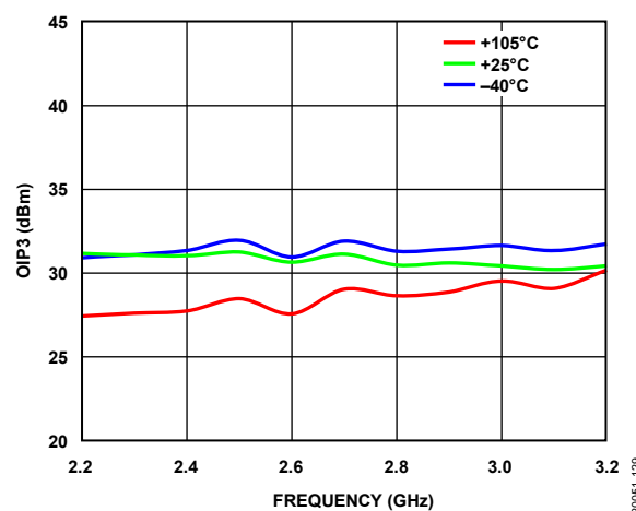
Figure 32. OIP3 vs. Frequency, 8 dBm Output Tone Power
