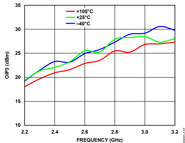
Figure 40. OIP3 vs. Frequency at Various Temperatures, -8 dBm Output Tone Power
