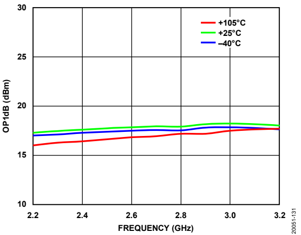
Figure 34. OP1dB vs. Frequency at Various Temperatures
