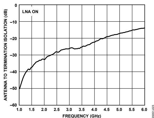
Figure 26. Antenna to Termination Isolation vs. Frequency, LNA On
