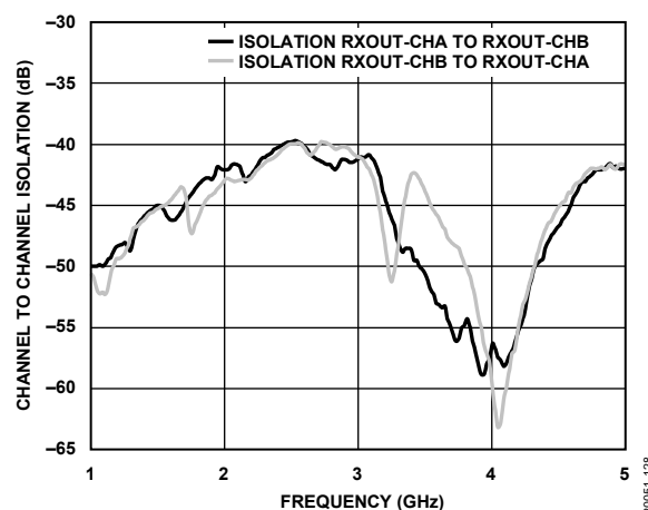
Figure 31. Channel to Channel Isolation vs. Frequency
