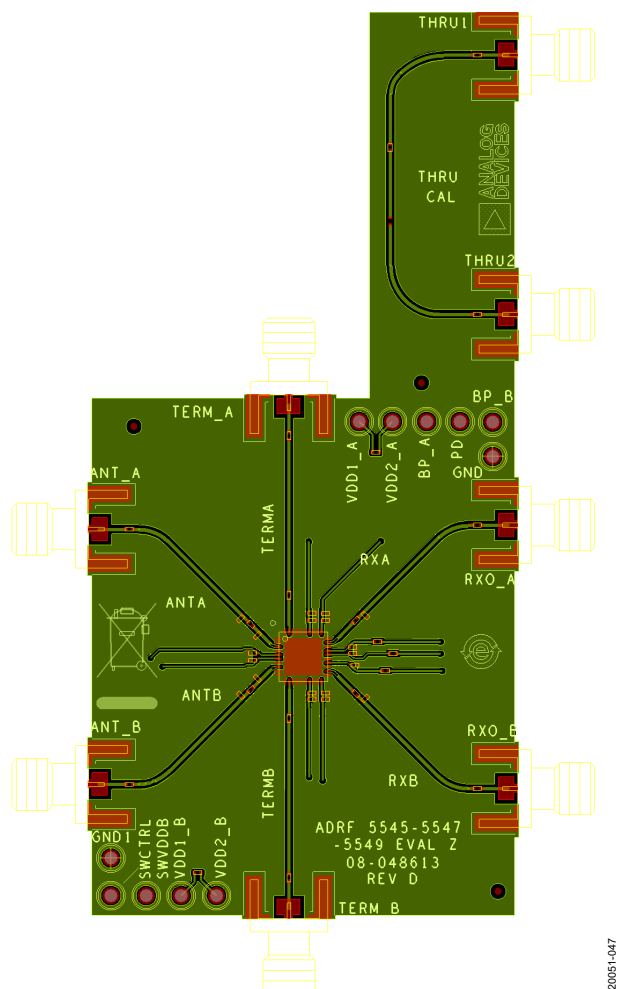
Figure 47. ADRF5545A-EVALZ Evaluation Board
