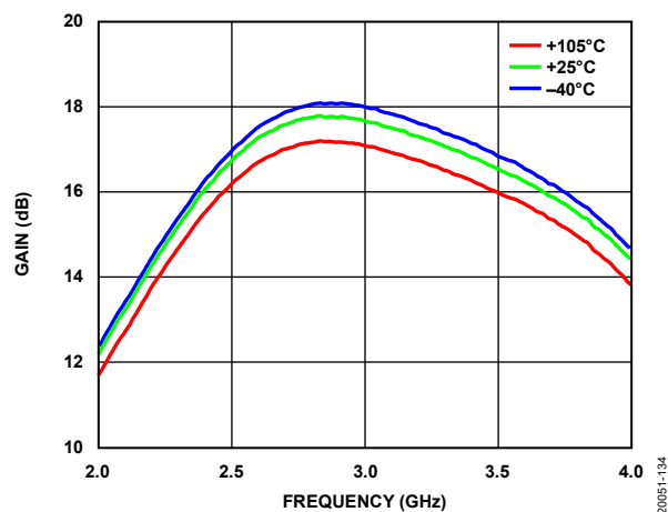
Figure 38. Gain vs. Frequency at Various Temperatures, 2.0 GHz to 4.0 GHz
