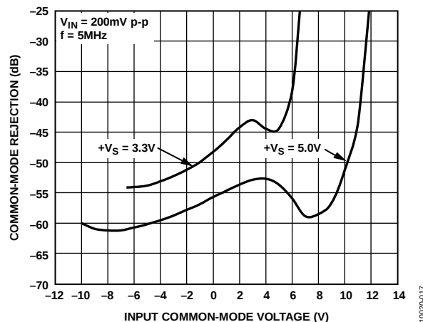
Figure 15. Small Signal CMR vs. V_{INCM} for Various Supply Voltages
