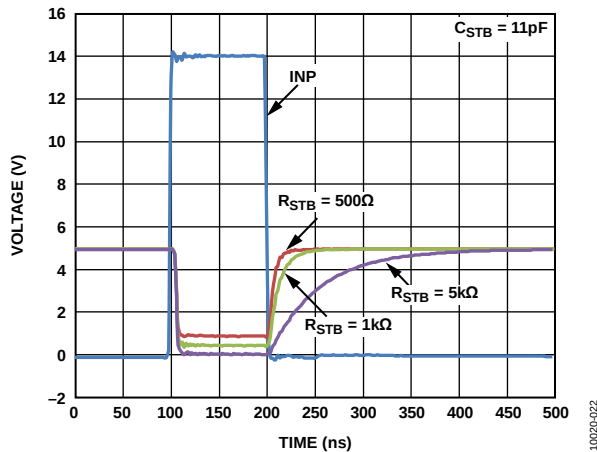
Figure 19. Short-to-Battery Output Flag Response for Various R_{STB} , ADA4830-1
