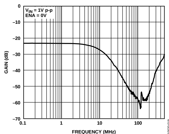
Figure 16. Input-to-Output Isolation with Device Disabled
