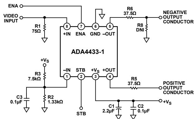
Figure 51. Example Compatible Schematic Configured for the ADA4433-1
